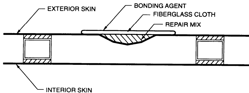
C - REPAIRED LARGE OR DEEP DENT.
