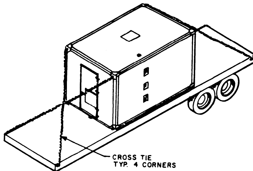
Figure 3-32. Truck Tiedown.
