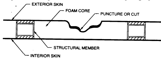
A - SMALL SINGLE SKIN PUNCTURE OR CUT IN SANDWICH CONSTRUCTION.
