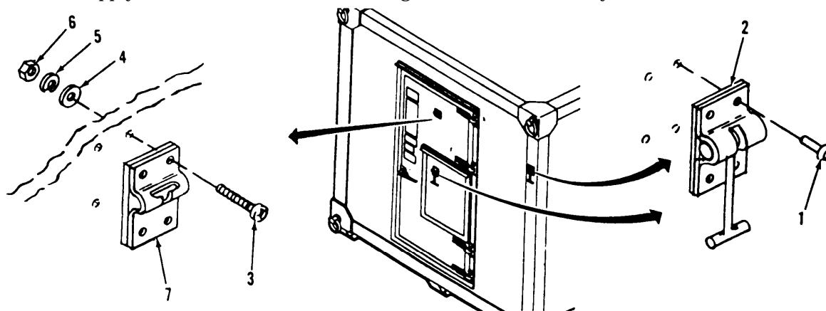
Figure 3-13. T-Latch Replacement.
